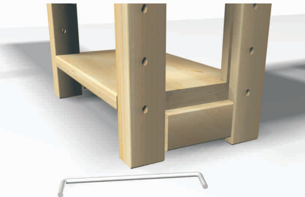
Without shelf support on bottom shelf (Only applicable if not using a fascia).
